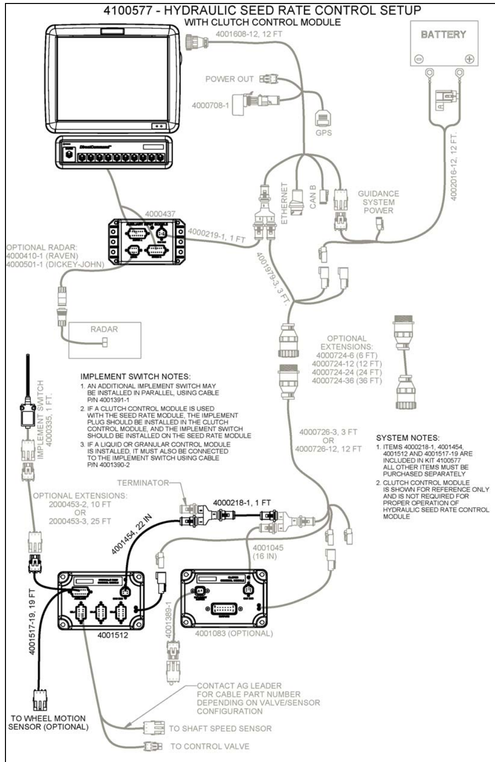
Figure 1. System Layout
